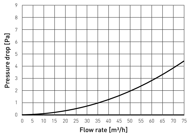
Specifications for supply and extraction
