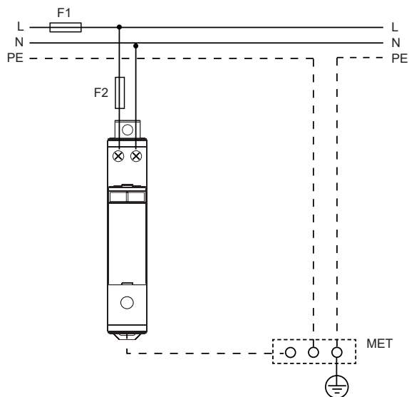
TN-S (with PE and Neutral distribution)
