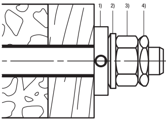
Pre-assembly with FIS A and injection system FIS SB Sizes: M12, M16, M20, M24
