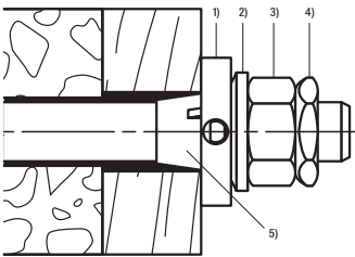
Push-through installation with FIS A and injection system FIS SB Sizes: M12, M16, M20, M24
