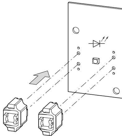
1b 1 - 2 M22-KP10, M22-KP01 + LED
