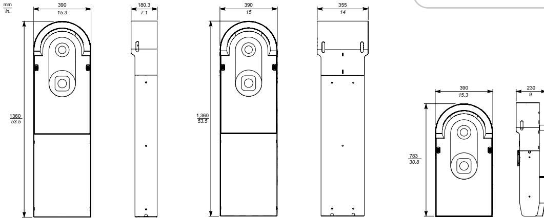
FS1CP: floor standing 1 charge point EVA1RFKS1
