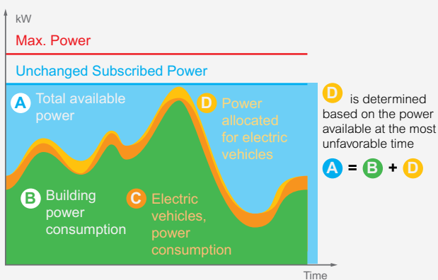
Static energy management: D is determined based on the available power at the most unfavorable time and is constant over time.
