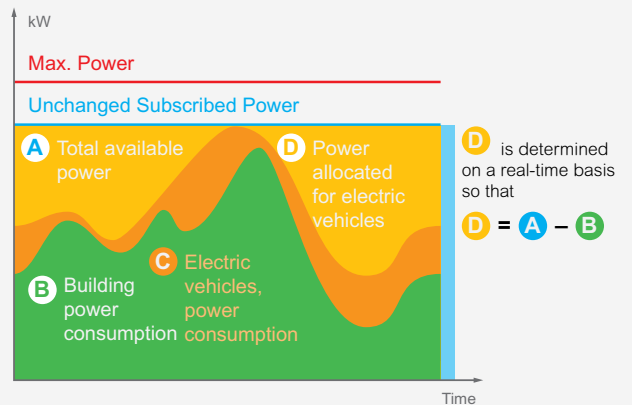
Dynamic energy management: setpoint "D" is adjusted in real time according to the consumption of the rest of loads in the building, to maximize the power allocated to charging electric vehicles.
