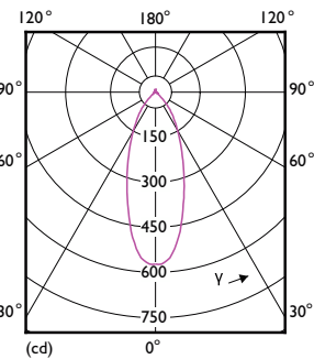
Light Distribution Diagram - MAS LEDspot UE 2.1-50W GU10 DIM 840 EELA
