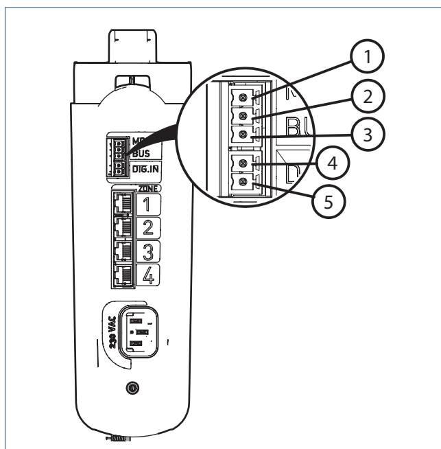
Multiconnector pitch 3.81 mm
