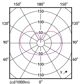
Light Distribution Diagram - MAS LEDBulbDT10.5-100W E27 CRI95A60CLG
