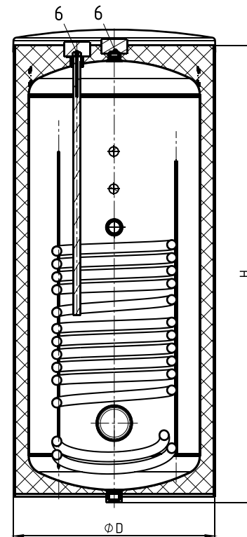
Section view B-B
