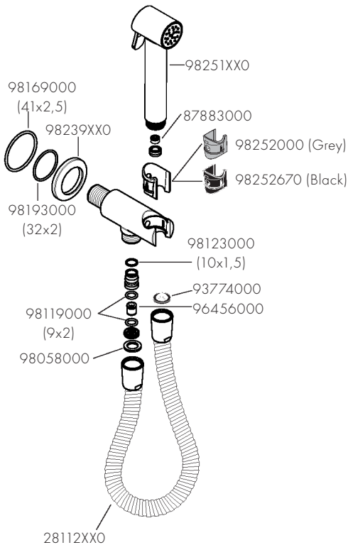
AXOR Bidette Showers 1jet round 29240XX0
