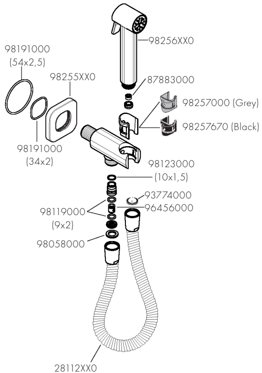
AXOR Bidette Showers 1jet softsquare 29241XX0
