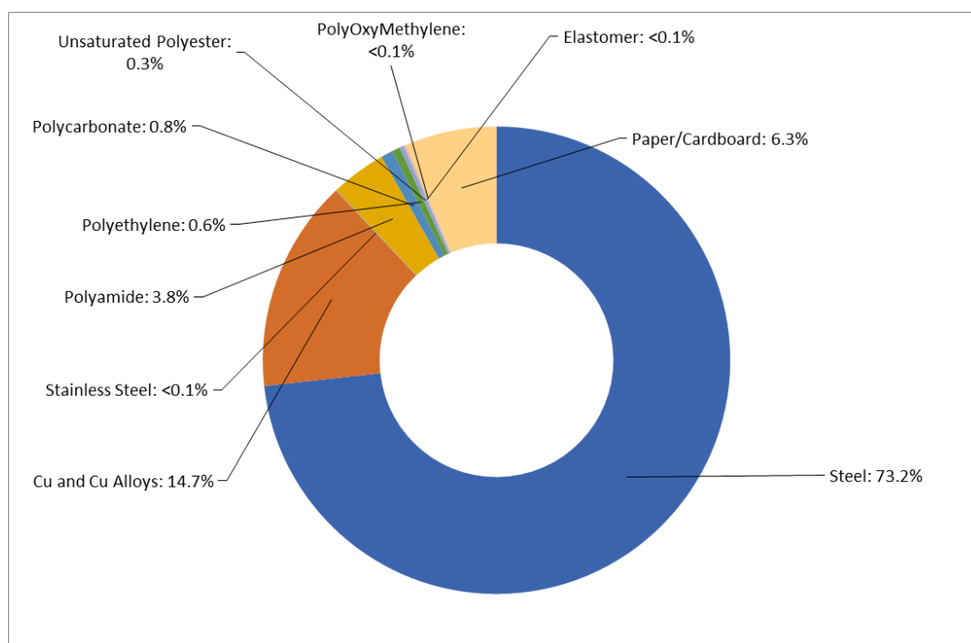
Figure 1: Composition of M E2.2-E6.2 220-250 Vac/dc
