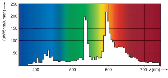
Spectral Power Distribution Colour - CDM-Rm Elite Mini 20W/830 GX10 MR16 10D
