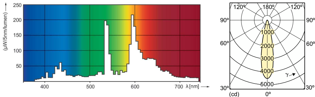
Spectral Power Distribution Colour - CDM-Rm Elite Mini 20W/830 GX10 MR16 25D
