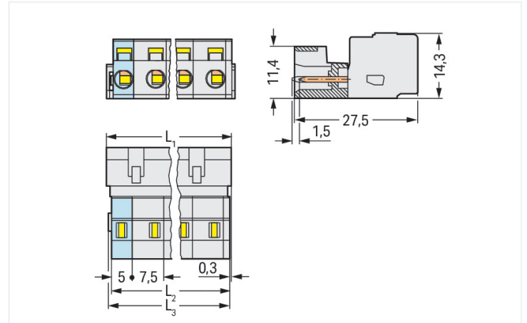
Dimensions in mm L1 = (\text{pole no.} - 1) \times \text{pin spacing} + 8.2 \text{ mm} L2 = L1 - 1.7 \text{ mm} L3 = L1 - 1.2 \text{ mm}
