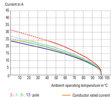
Derating Curve 2-conductor female connector (721-2202/026-000) with THT male header (721-262/001-000) Pin spacing: 7.5 mm / Conductor cross-section: 2.5 mm 2 "f-st" Based on: EN 60512-5-2 / Reduction factor: 0.8
