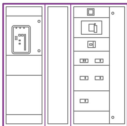
Standard configuration compliant with the construction and performance requirements of IEC 61439-2
