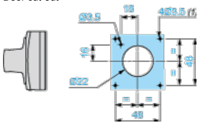
Door cut-out
