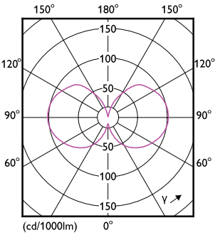
Light Distribution Diagram - MAS LEDBulbND5.2-75W E27 827 A60 FR G UE
