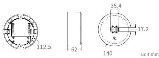
Surface Mount
