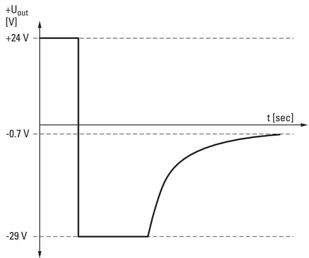
Figure 60: Voltage limiting when switching off inductive loads
