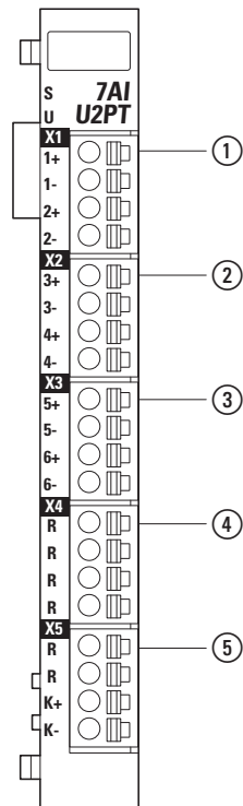
Figure 94: Pin assignment
