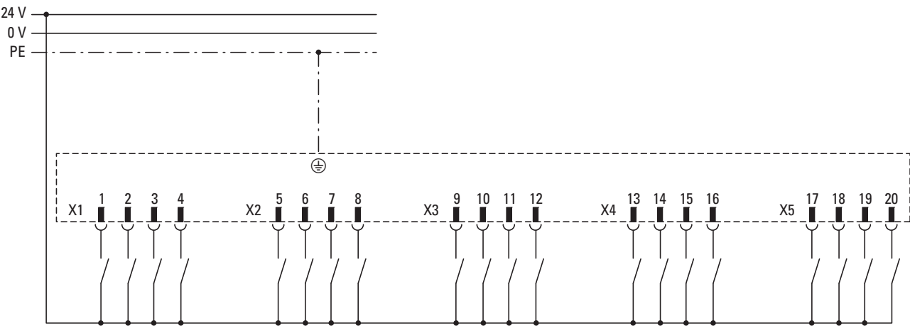
Figure 40: Input wiring
