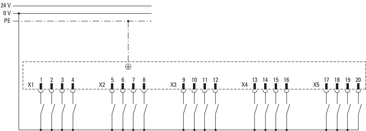
Figure 44: Input wiring
