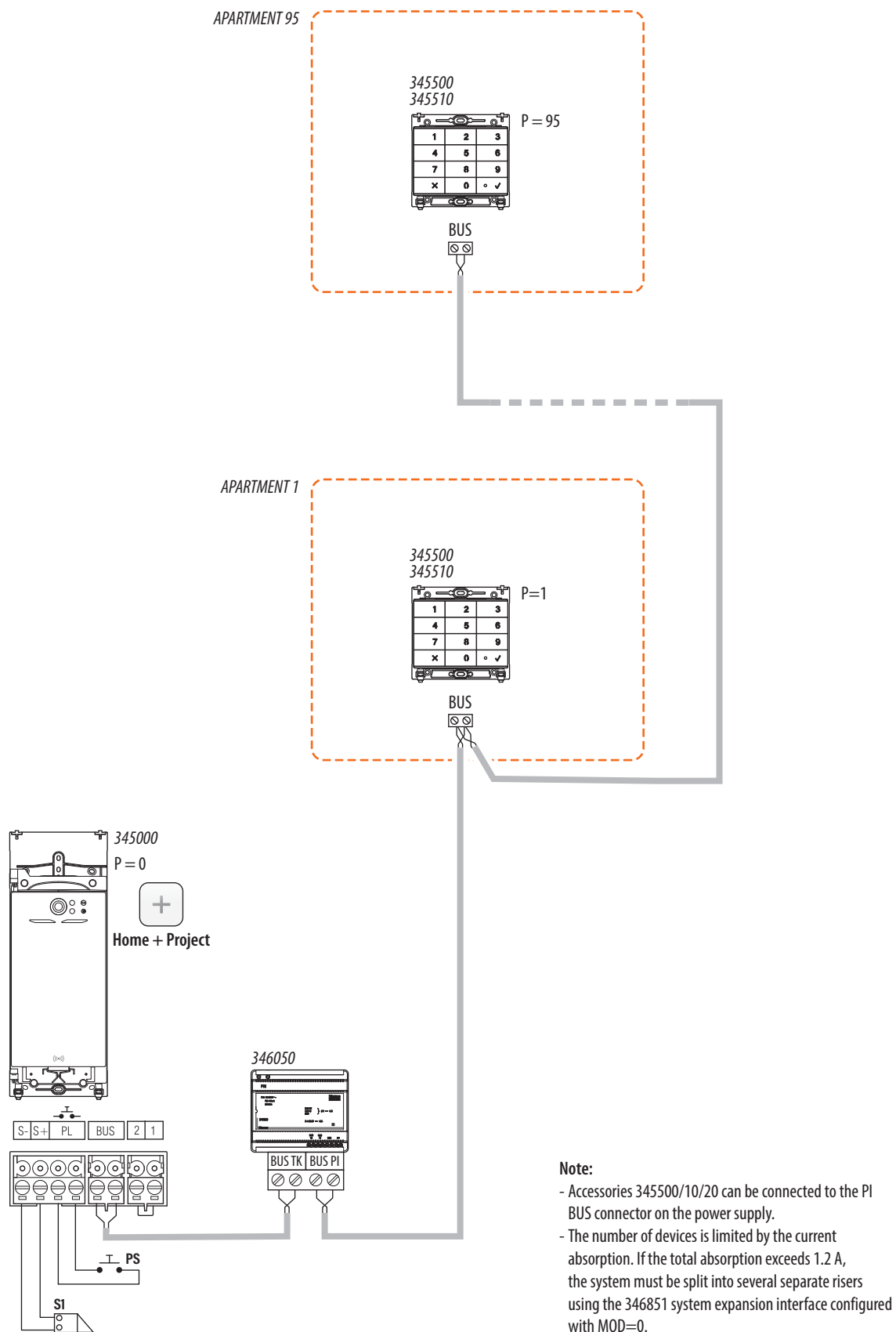
DIAGRAM 2 – EXAMPLE OF RESIDENTIAL SYSTEM FOR UP TO 95 APARTMENTS, WITH 1 ACCESSORY PER APARTMENT (WITHOUT INTERNAL UNIT)
