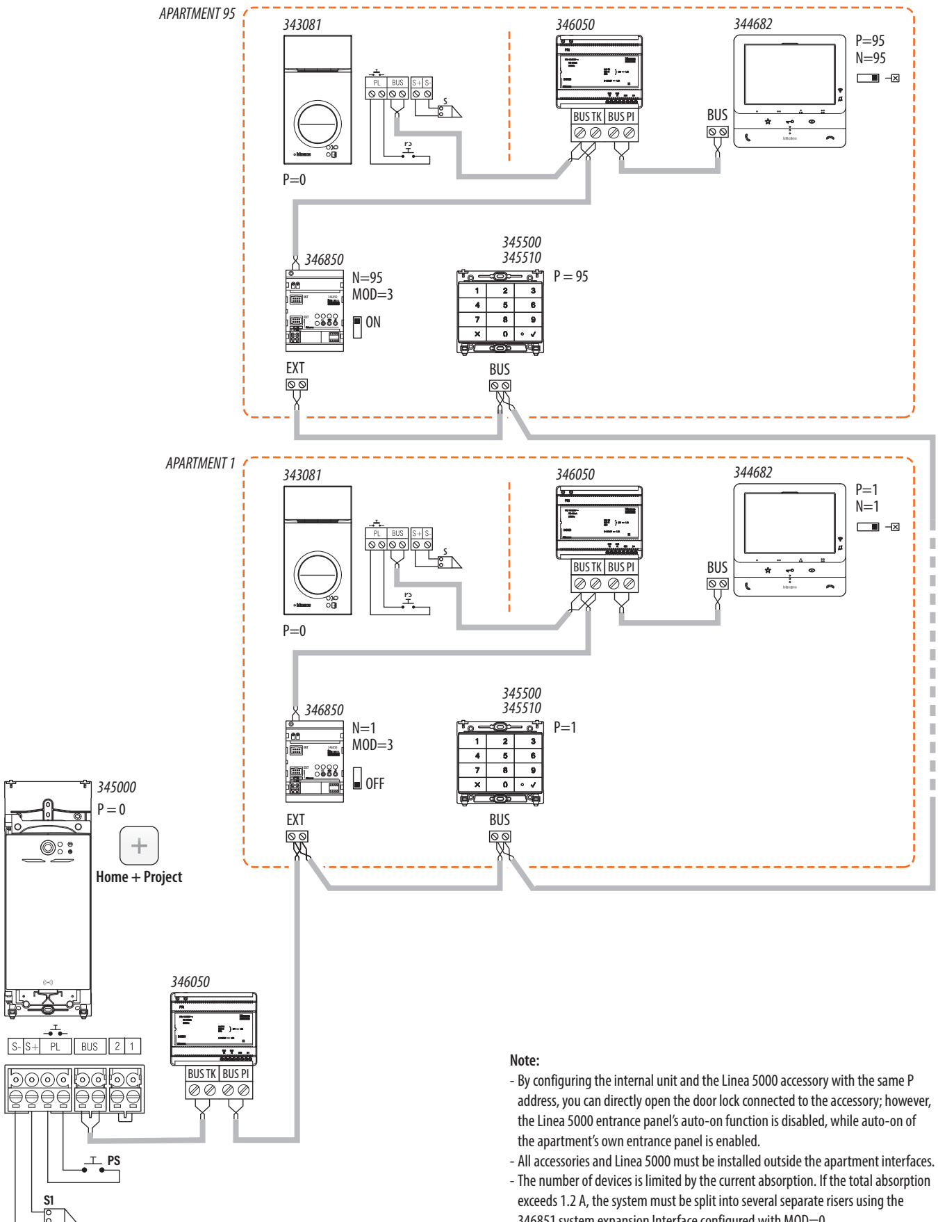
DIAGRAM 3 – EXAMPLE OF RESIDENTIAL SYSTEM FOR UP TO 95 APARTMENTS, EACH WITH 1 APARTMENT INTERFACE AND 1 ACCESSORY
