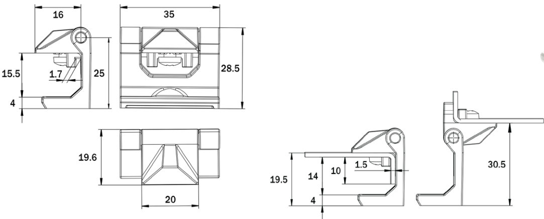
Hinge enables opening angle for door of 180 degrees.
