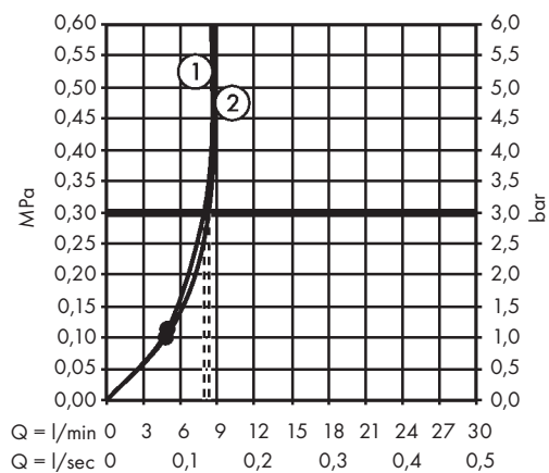
Crometta S 240 1jet Showerpipe Reno EcoSmart 27270000
