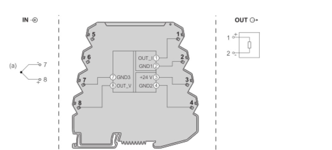
(a) : Thermocouple
