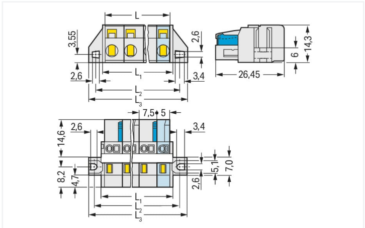
Dimensions in mm L = (pole no. – 1) x pin spacing + 5 mm L1 = L + 3 mm L2 = L + 8.8 mm L3 = L + 14.8 mm
