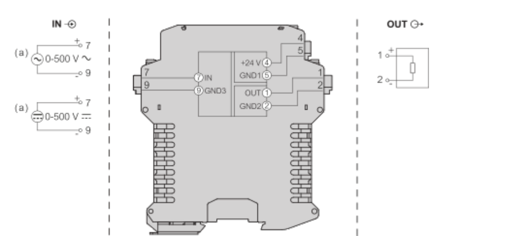
(a) : AC/DC Voltage Source
