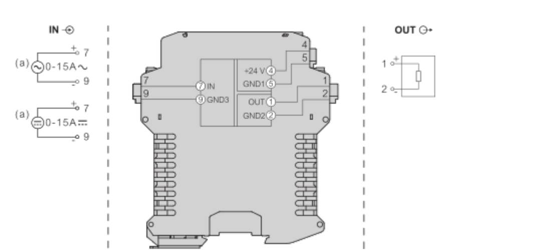
(a) : AC/DC Current Source
