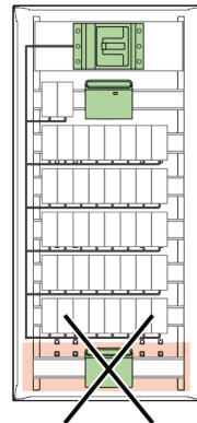
Illustration 6: NSX/NSXm on a mounting plate at the top of the W600/W850 (With or without incoming connection block)
