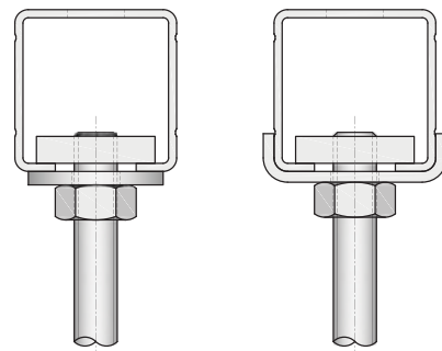
Picture 4: Increase rigidity for loads beneath the rail by using U-shaped washers (right picture) instead of standard flat washers (left picture)
