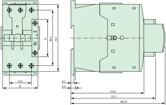
Contactors DILM40-DILM65
