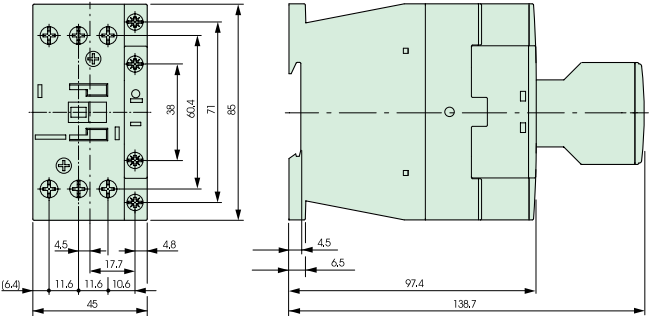
Contactors DILM17-DILM32
