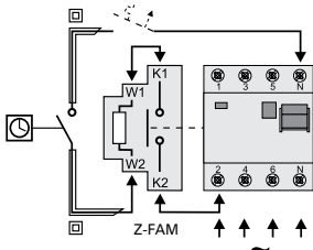
Connection diagram: RCCB-4p, RCCB feed below
