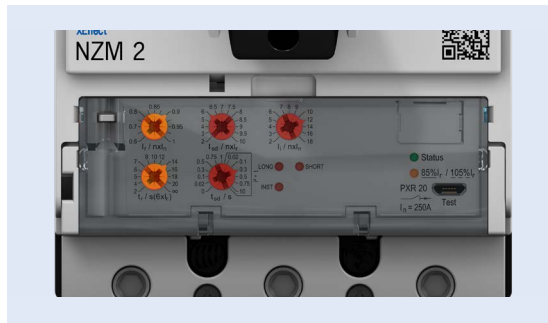
9. The NZM protects special applications with high switching capacities at 690 V AC, at high frequencies, in IT networks, and at 1000 V AC. See page 35
