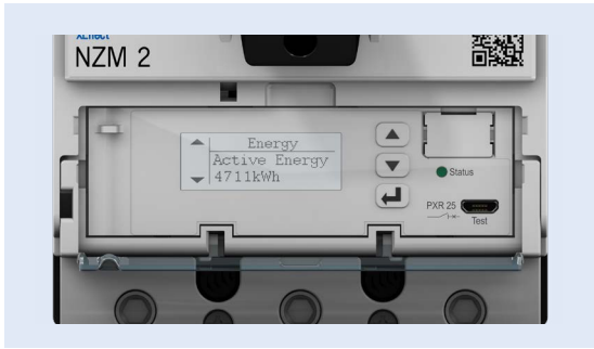
10. The NZM offers protection and ISO 50001 energy metering with Class 1 accuracy* in accordance with IEC 61557-12. See page 38
