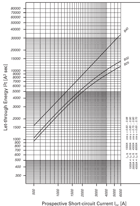
Let-through Energy AFDD+, Characteristic B, 2-pole, 25-40 A
