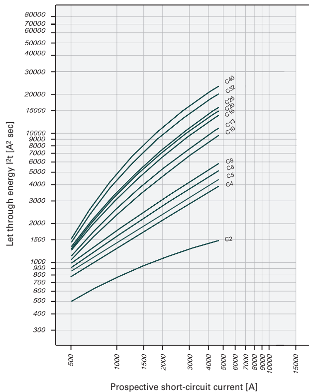
Let-through Energy PKN4, Characteristic C, 1+N-pole
