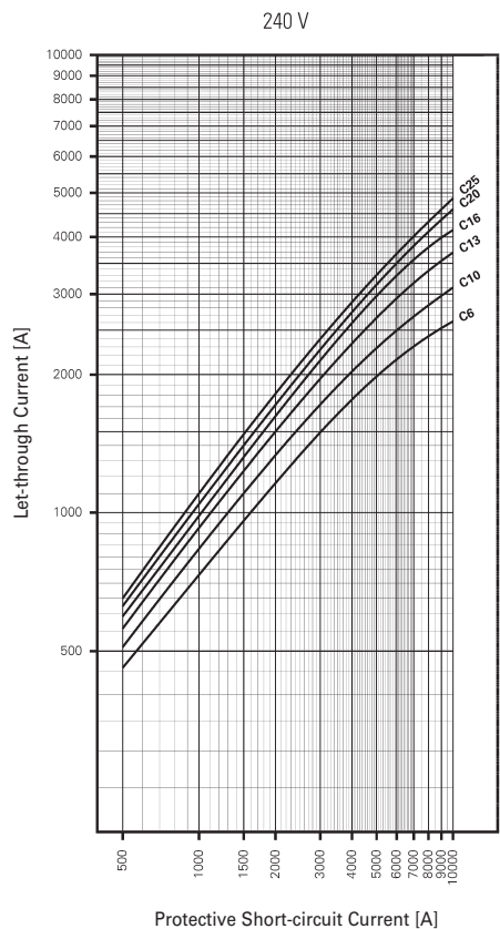
Let-through Current dRBM, Characteristic C
