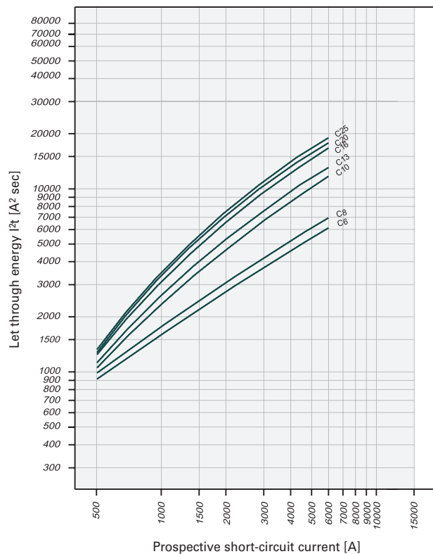
Let-through Energy PFL6, Characteristic C, 1+N-pole
