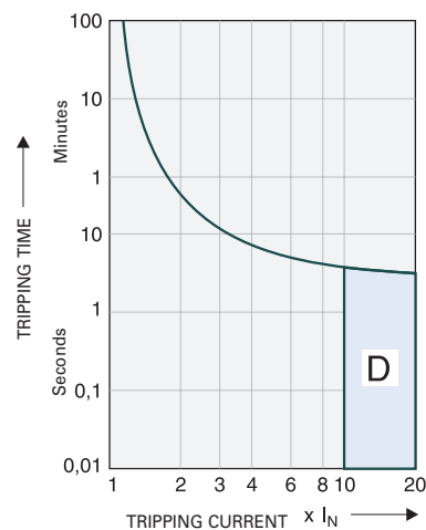
Tripping characteristic D
