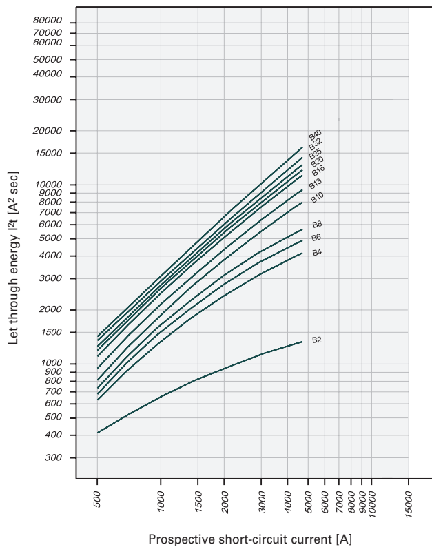
Let-through Energy PKN4, Characteristic B, 1+N-pole
