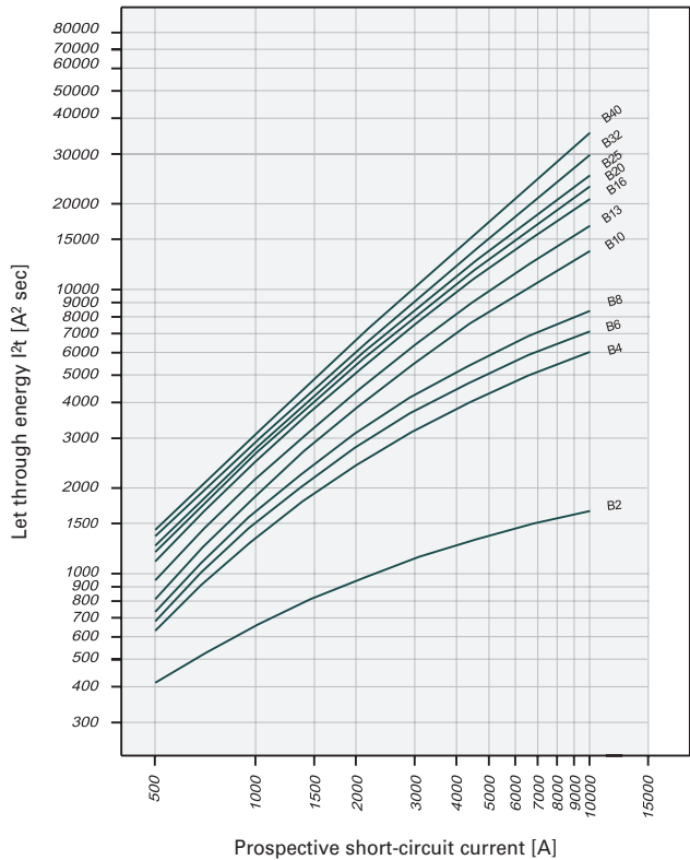
Let-through Energy PKNM, Characteristic B, 1+N-pole
