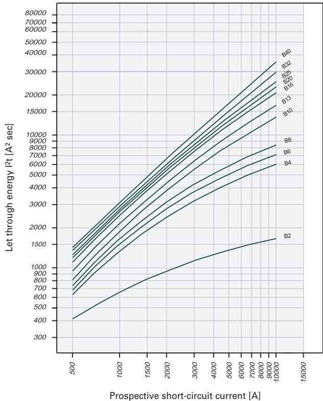
Let-through Energy PFL7, Characteristic B, 1+N-pole
