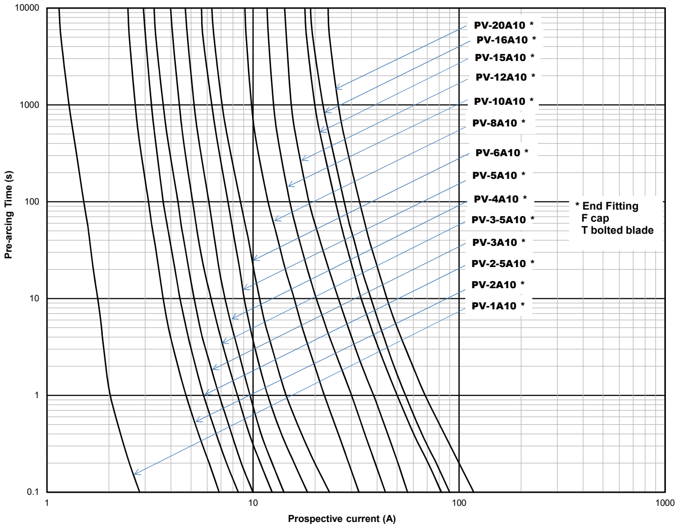
Time-current curve - 1 A to 20 A
