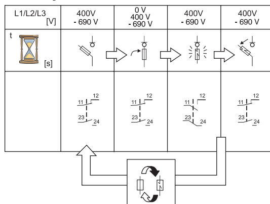
Function diagram
