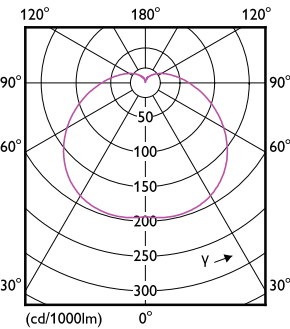
Light Distribution Diagram - CorePro LEDbulb ND 13-100W A60 E27 830
