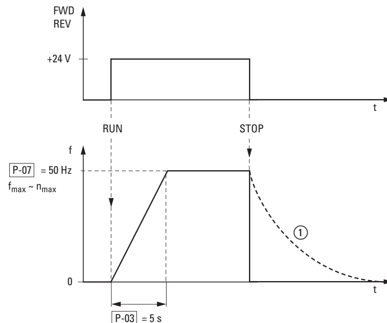
Figure 51: Start-stop command at maximum set point voltage, acceleration ramp 5 s
