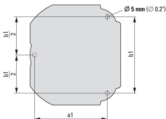
Figure 31: Mounting dimensions
