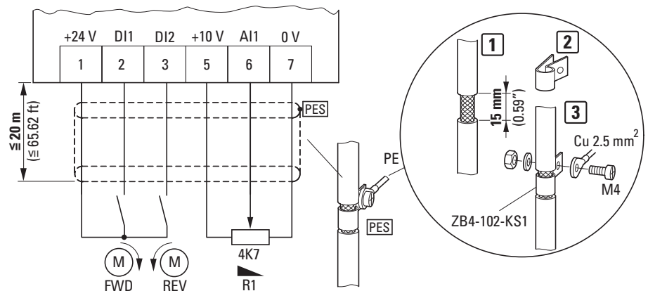
Figure 40: Simple connection example
