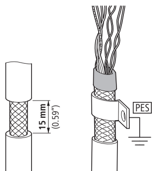
Figure 41: Screen termination at one end (PES) close to the variable frequency drive
