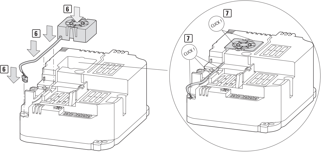
Figure 24: Install the new fan
