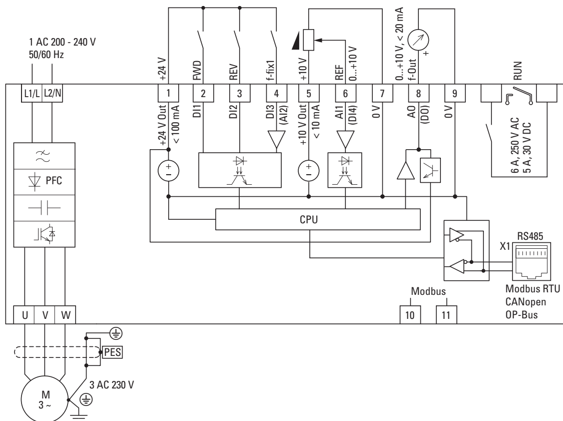
Figure 48: Block diagram DB1-127D0FN-N2CC-PFC
