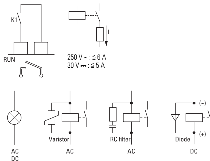
Figure 42: Connection examples with suppressor circuit
