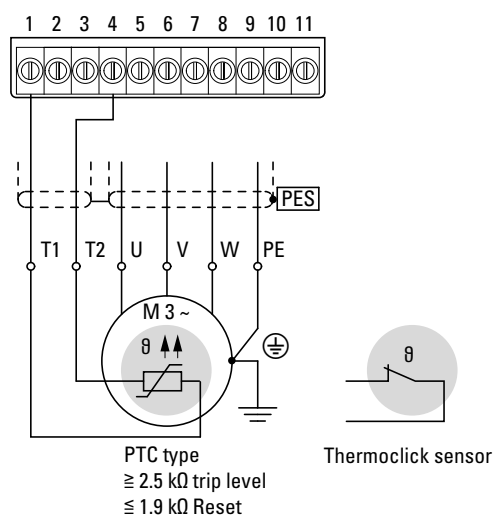
Figure 44: Thermistor connection
