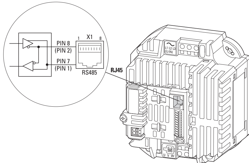
Figure 43: RJ45 interface
