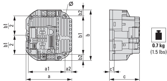
Figure 53: Dimensions
