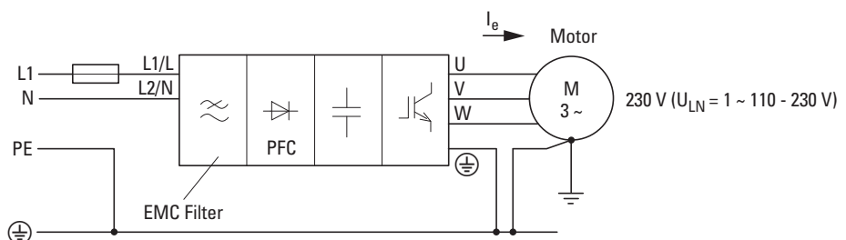
Figure 11: DB1-1M...
