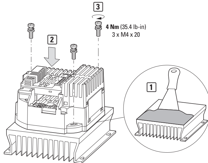
Figure 30: Cooling measures
