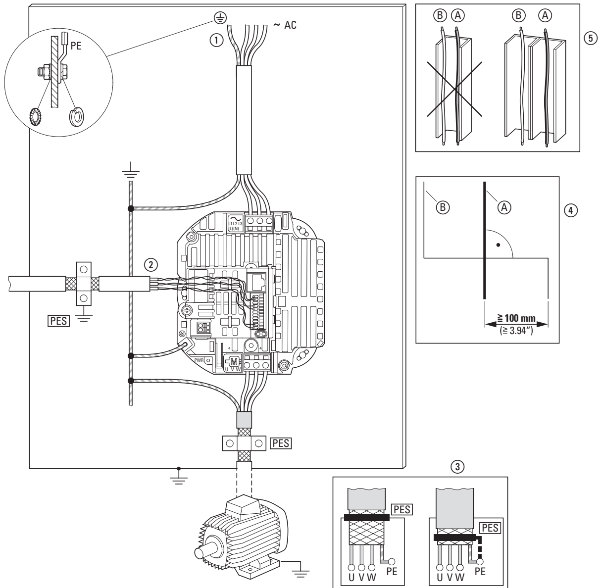
Figure 34: Correct EMC installation
