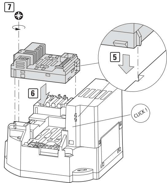
Figure 21: Put on the control board
