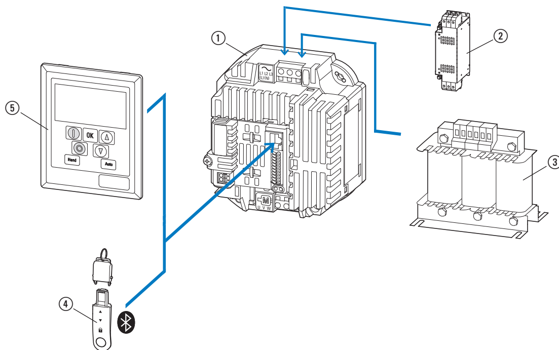
Figure 2: System overview
