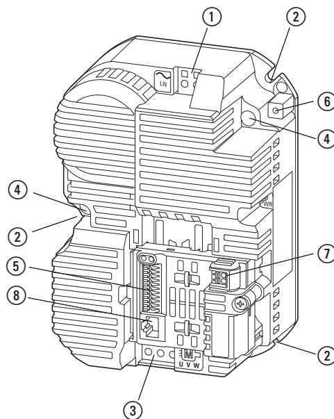
Figure 8: Parts designation – with frame size FS1C
